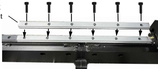
Bearing rail joint
